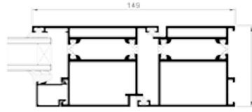
Door - cross-section
